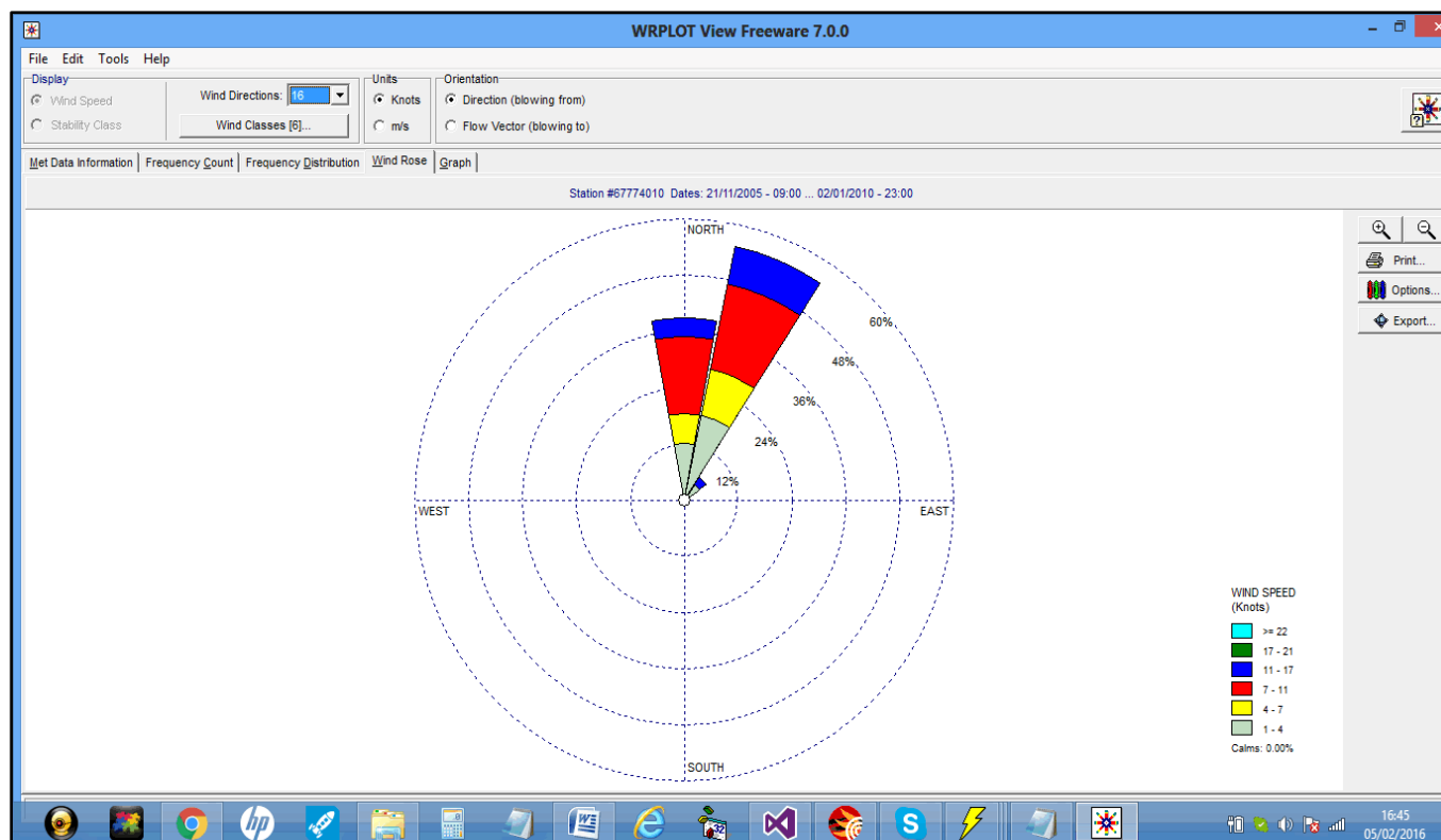
Figure 81: Windrose plot
