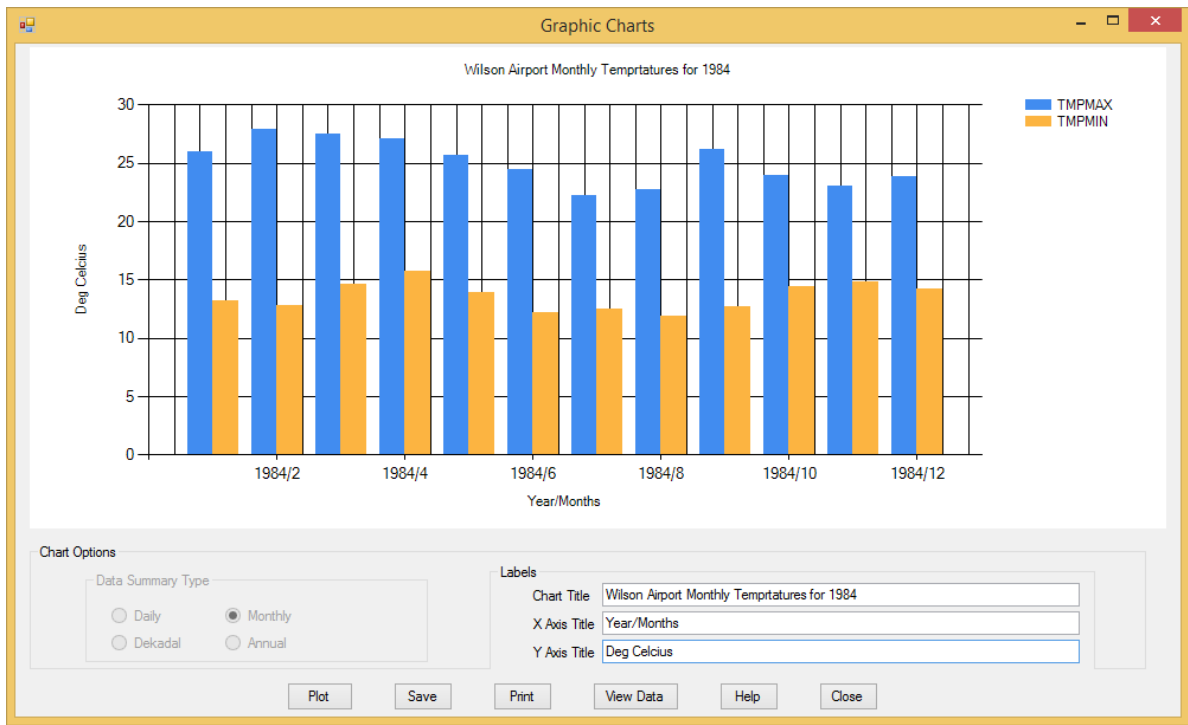
Figure 83: Temperatures Histograms
